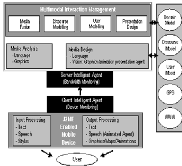
Figure 1: TeleMorph Architecture
