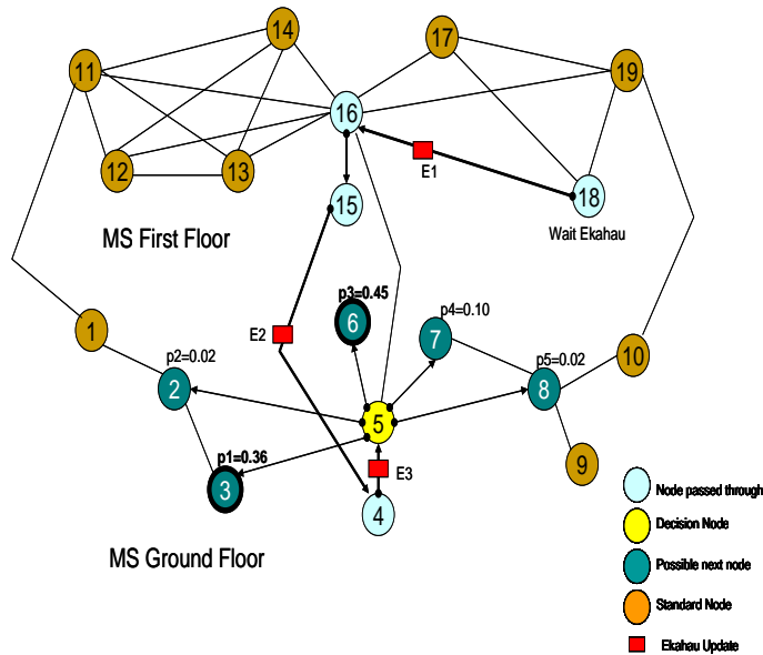
Figure 9: Probability from Temporal Fuzzy Rule
