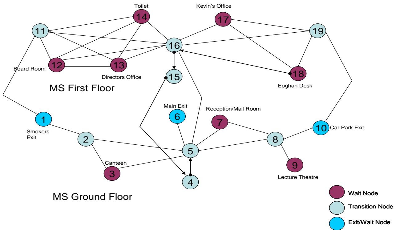
Figure 5: MS building represented as a graph
