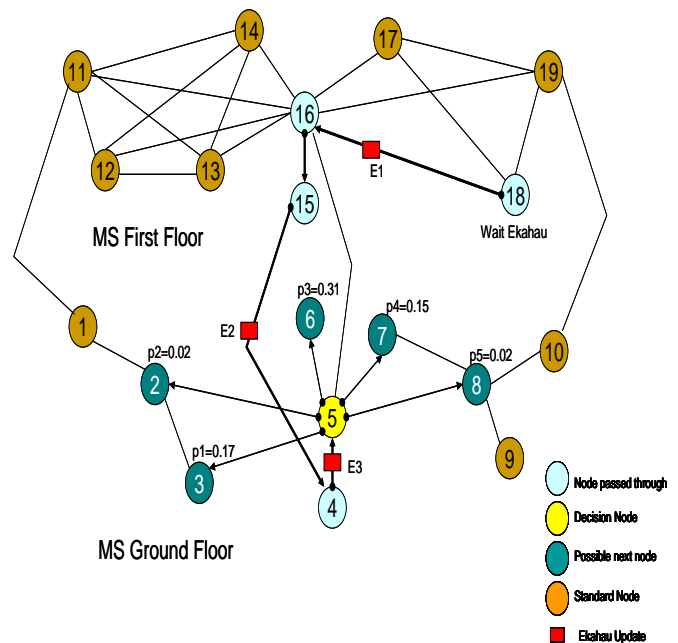
Figure 8: Probability from Bayesian Filter
