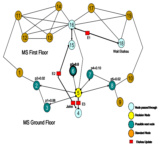
Figure 10: Probability from Other User Fuzzy Rule
